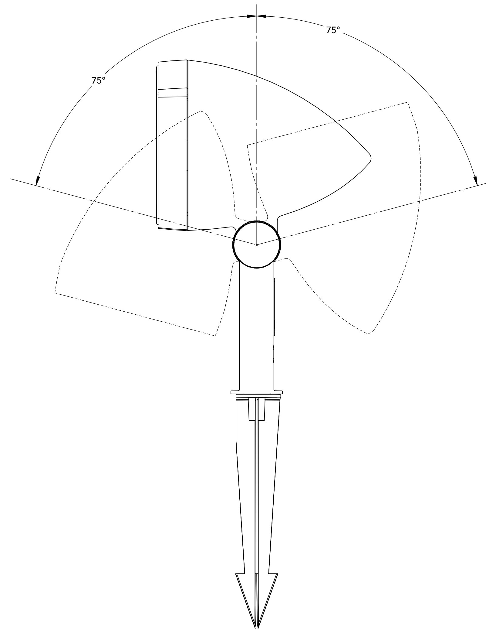
SIDE
