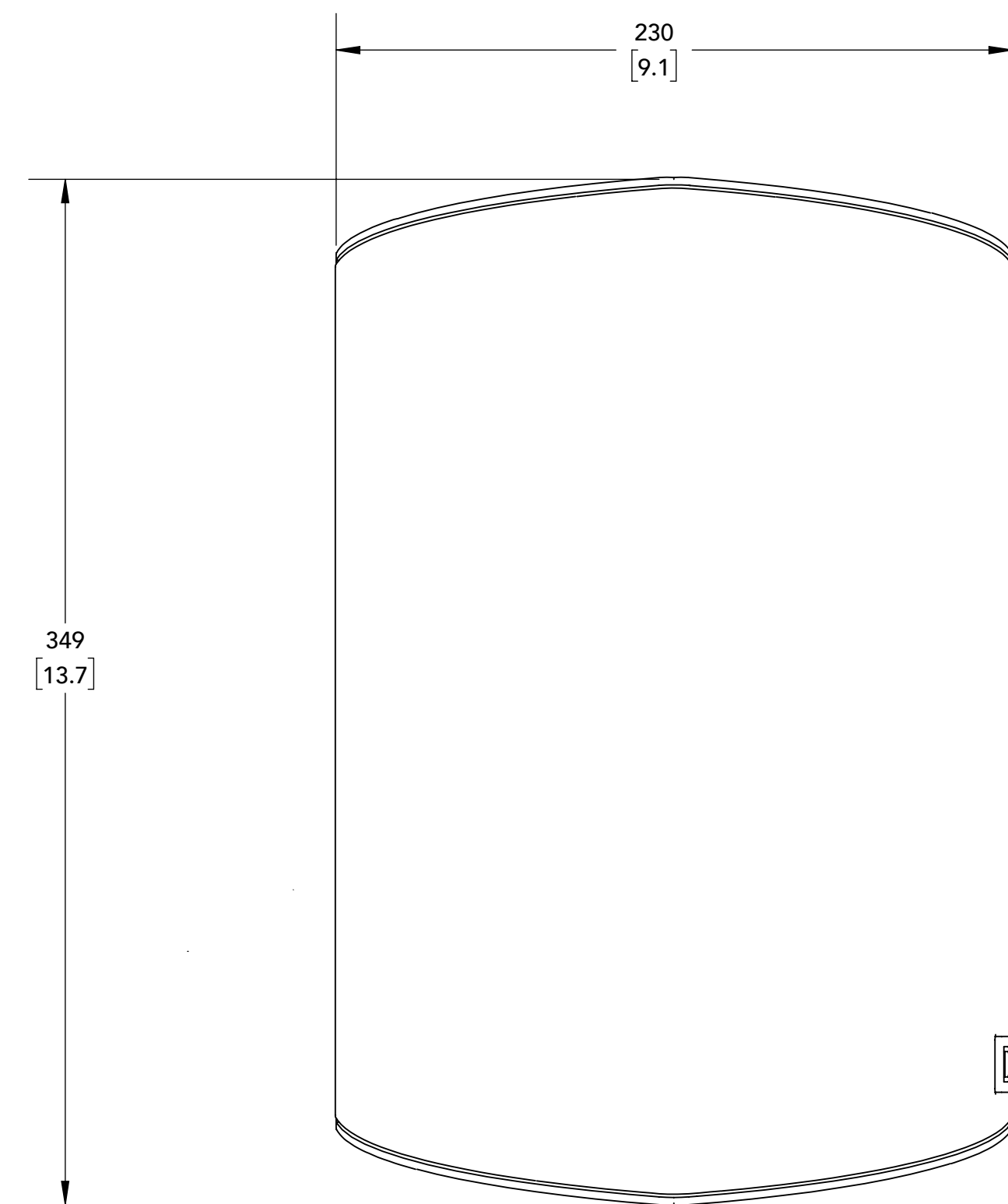
FRONT
